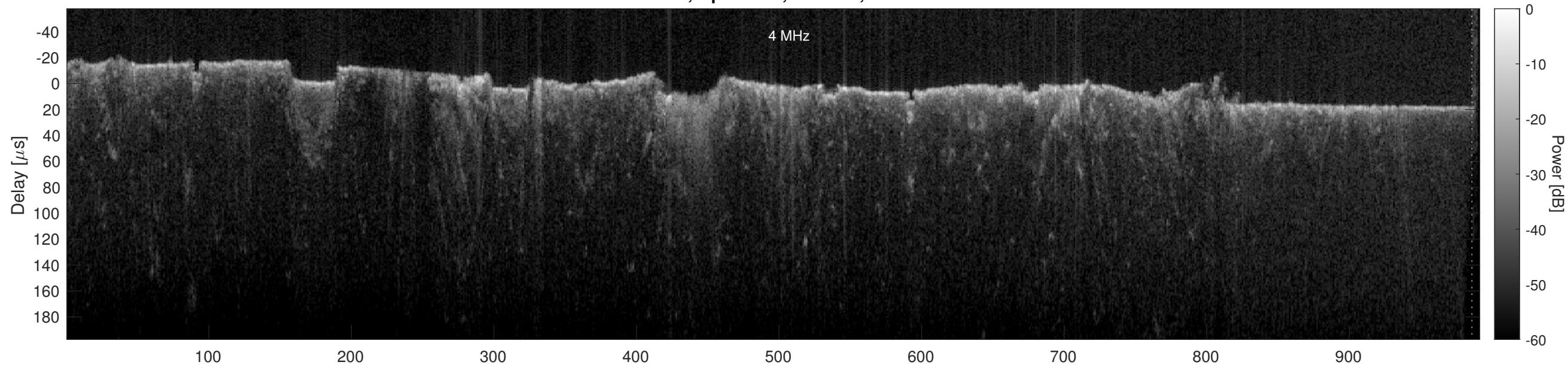
Orbit 14423, Optimized, Window, Channel 2
