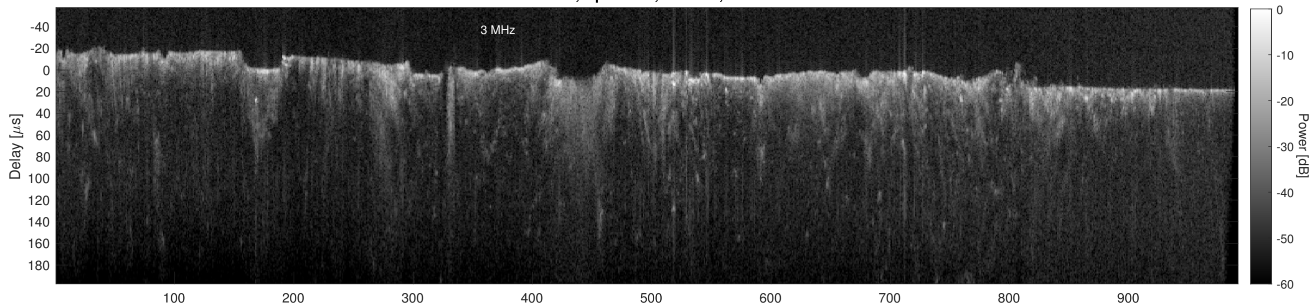
Orbit 14423, Cluttergram
