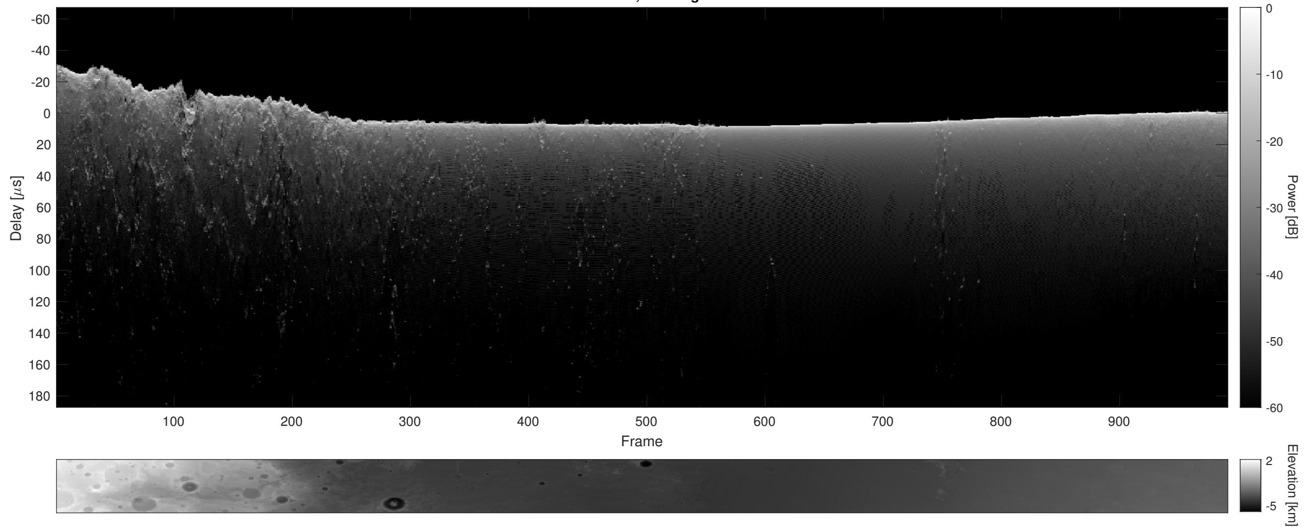
Orbit 14425, Cluttergram
