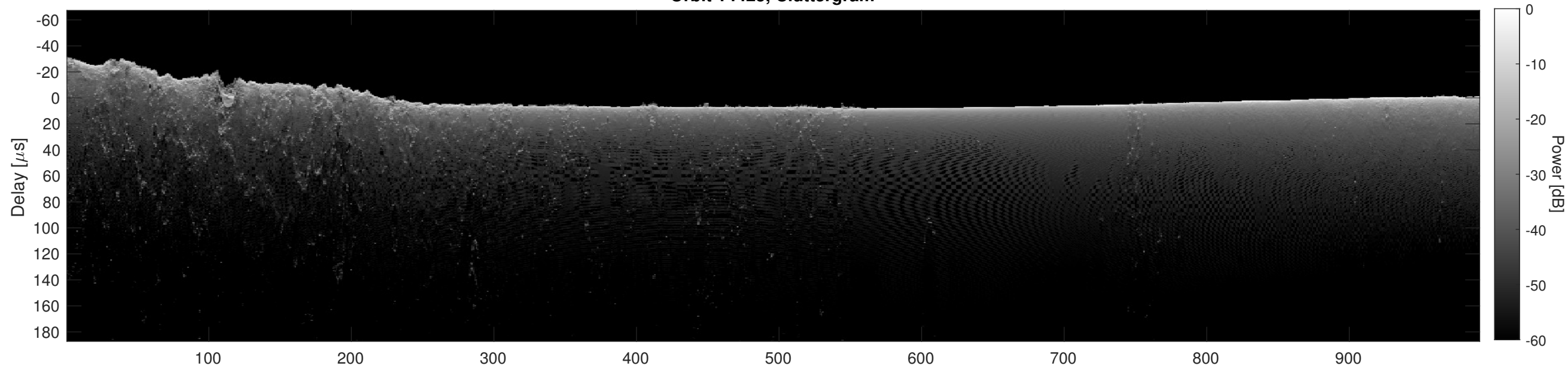
Orbit 14425, Cluttergram
