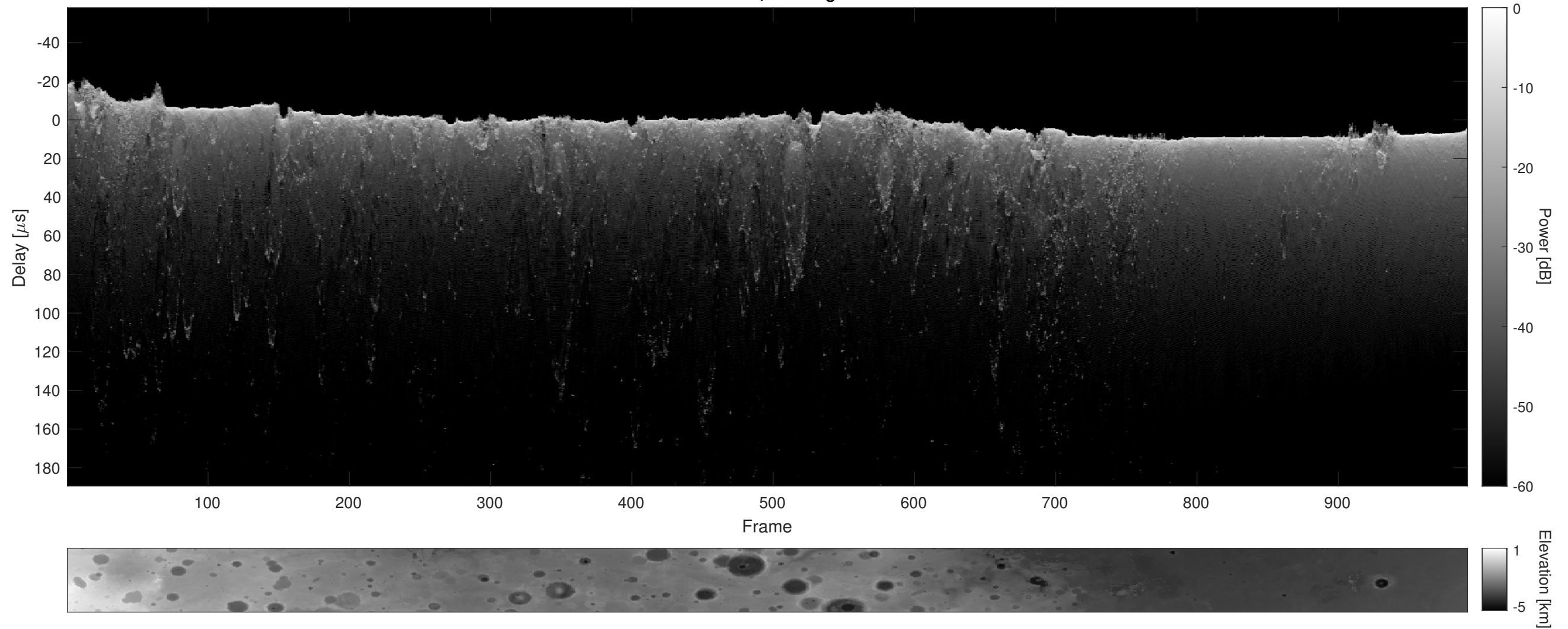
Orbit 14427, Cluttergram
