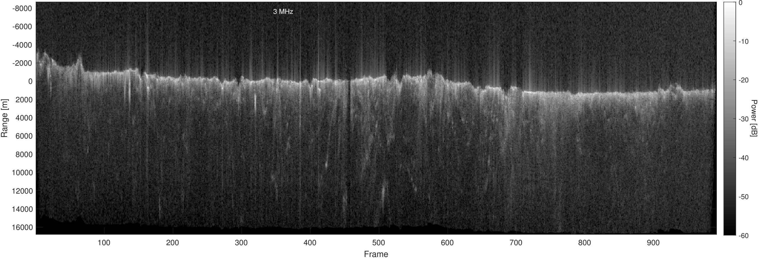
Orbit 14427, Optimized, No Window, Depth-Corrected, Channel 2
