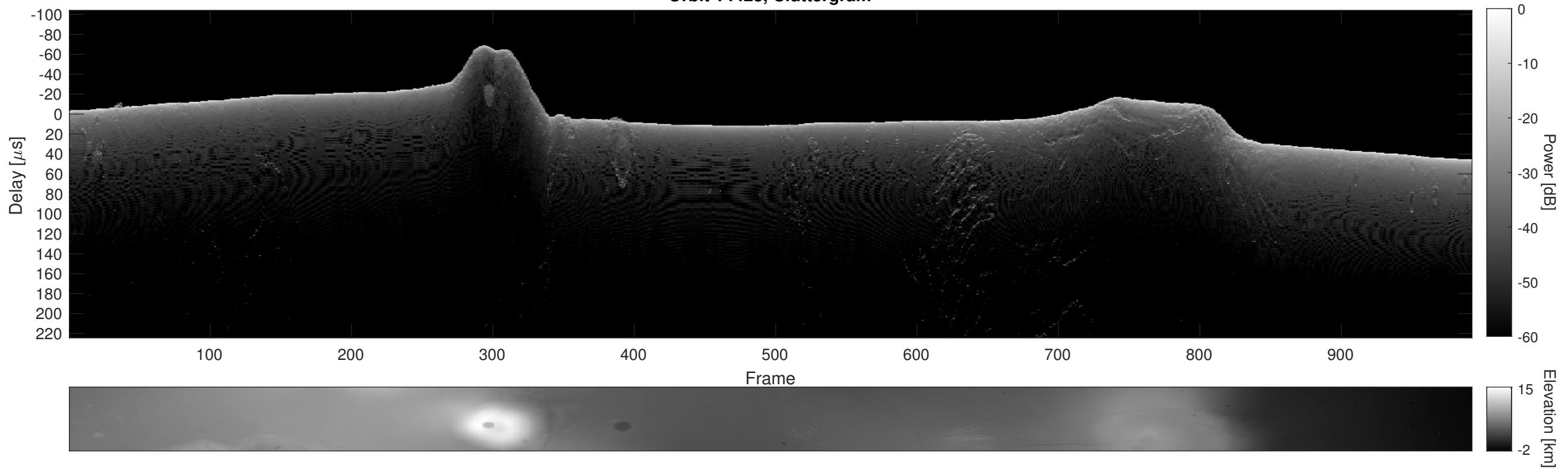
Orbit 14428, Cluttergram
