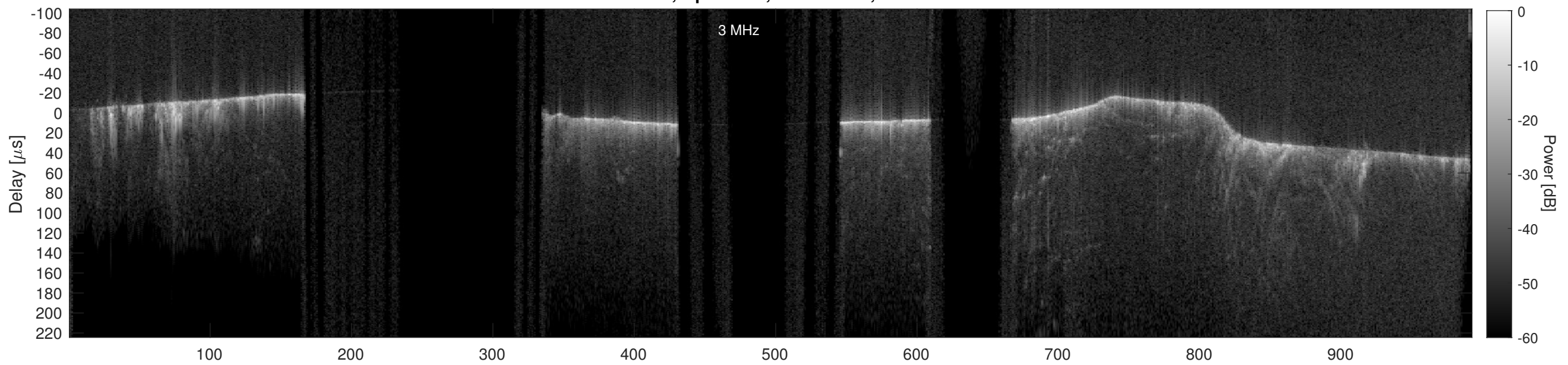
Orbit 14428, Cluttergram
