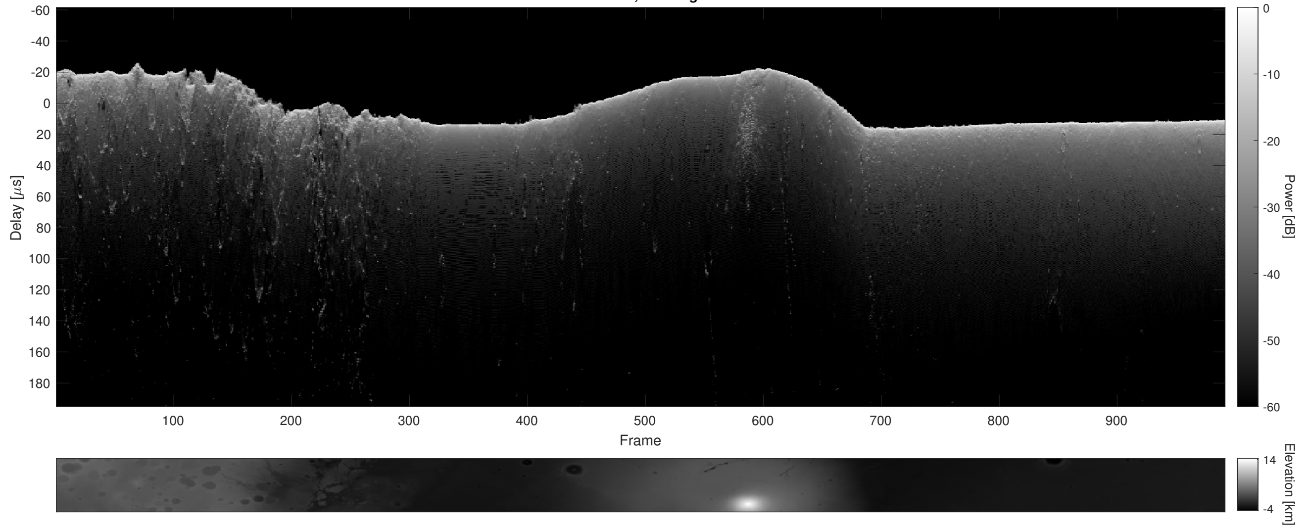
Orbit 14429, Cluttergram
