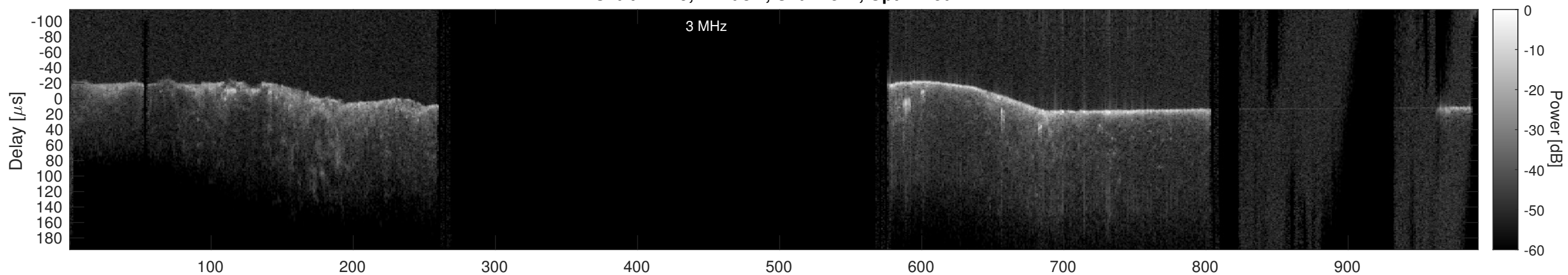
Orbit 14429, Cluttergram
