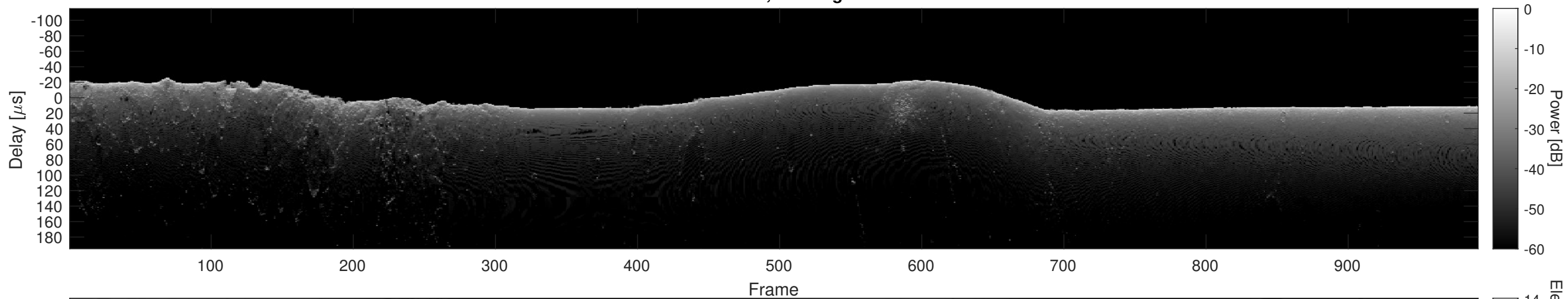
Orbit 14429, Cluttergram
