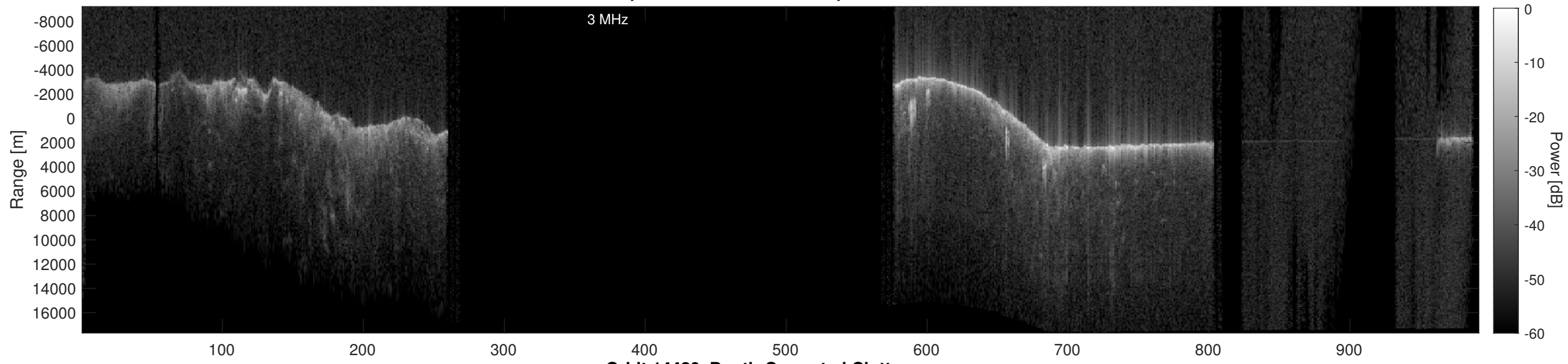
Orbit 14429, Depth-Corrected Cluttergram
