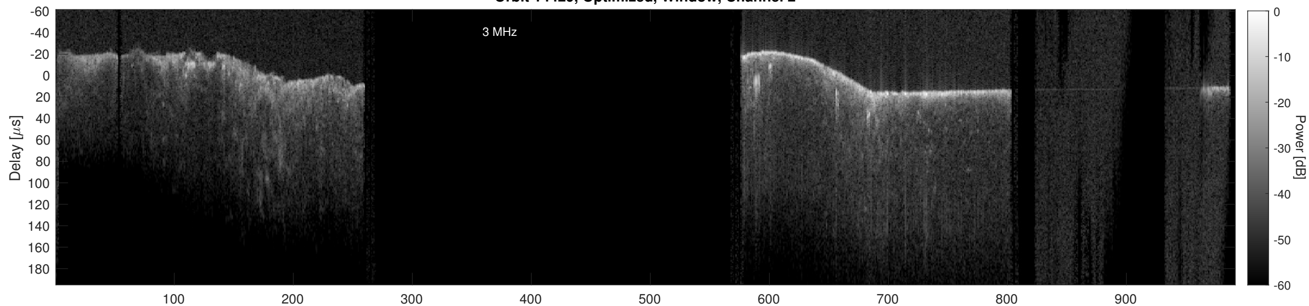
Orbit 14429, Cluttergram
