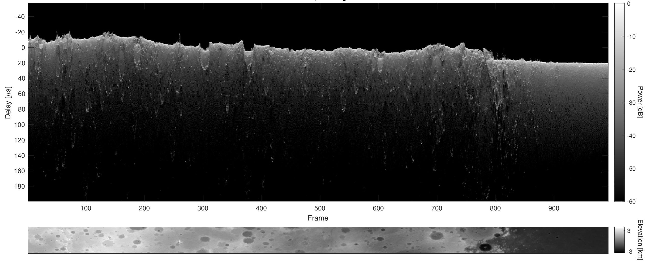
Orbit 14430, Cluttergram
