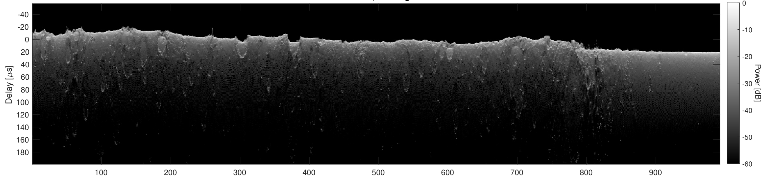
Orbit 14430, Cluttergram
