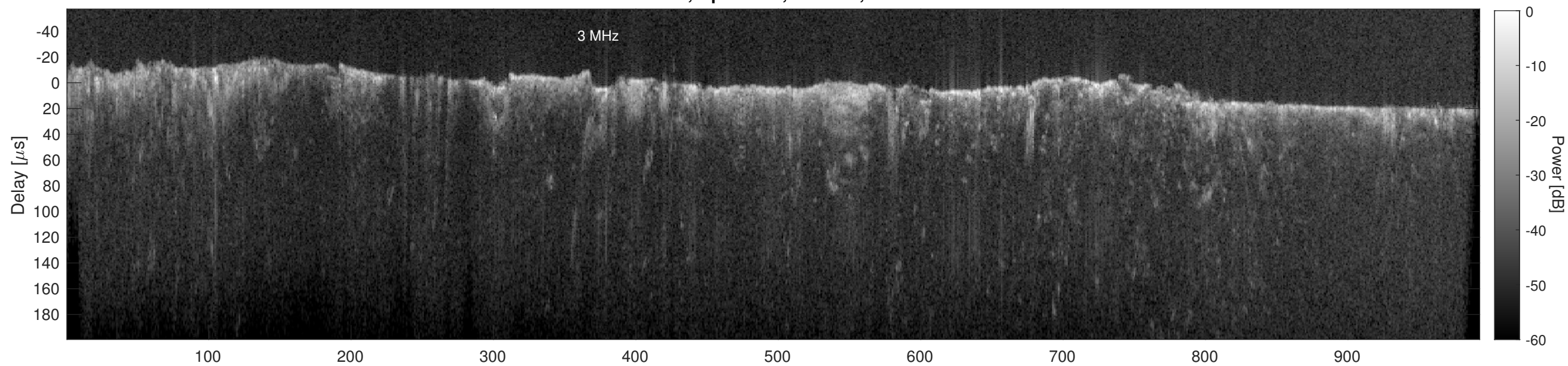
Orbit 14430, Cluttergram
