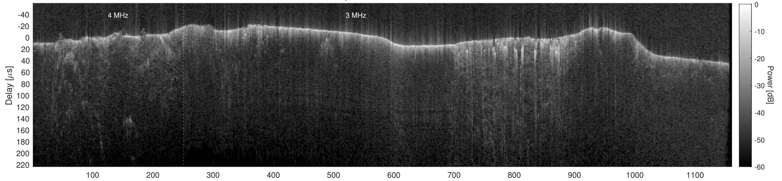
Orbit 14435, Cluttergram
