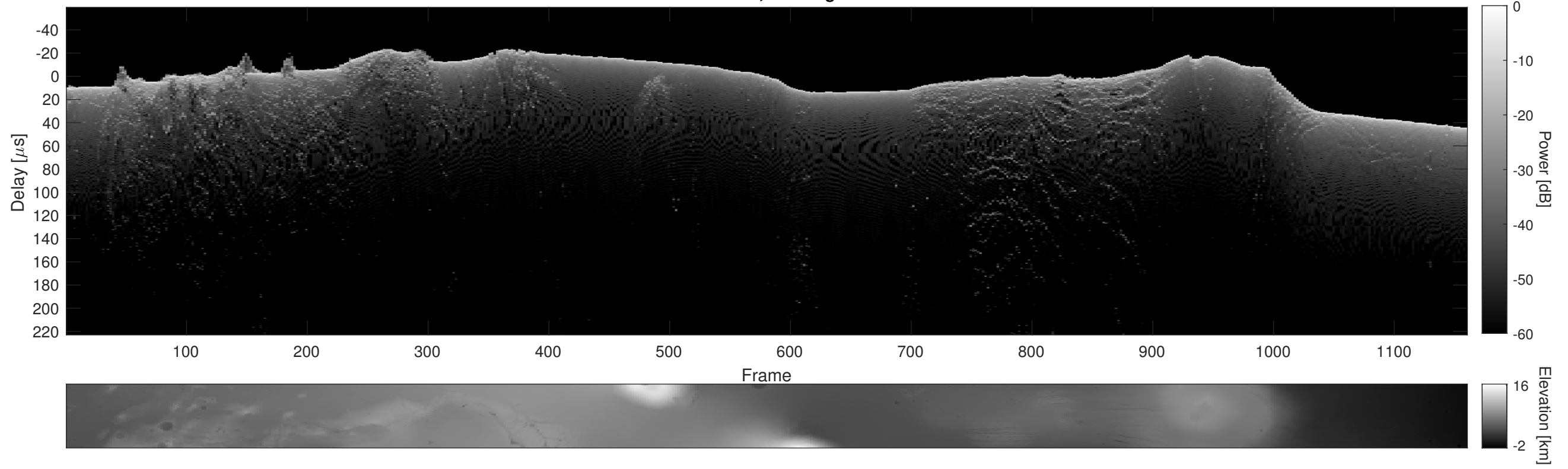
Orbit 14435, Cluttergram
