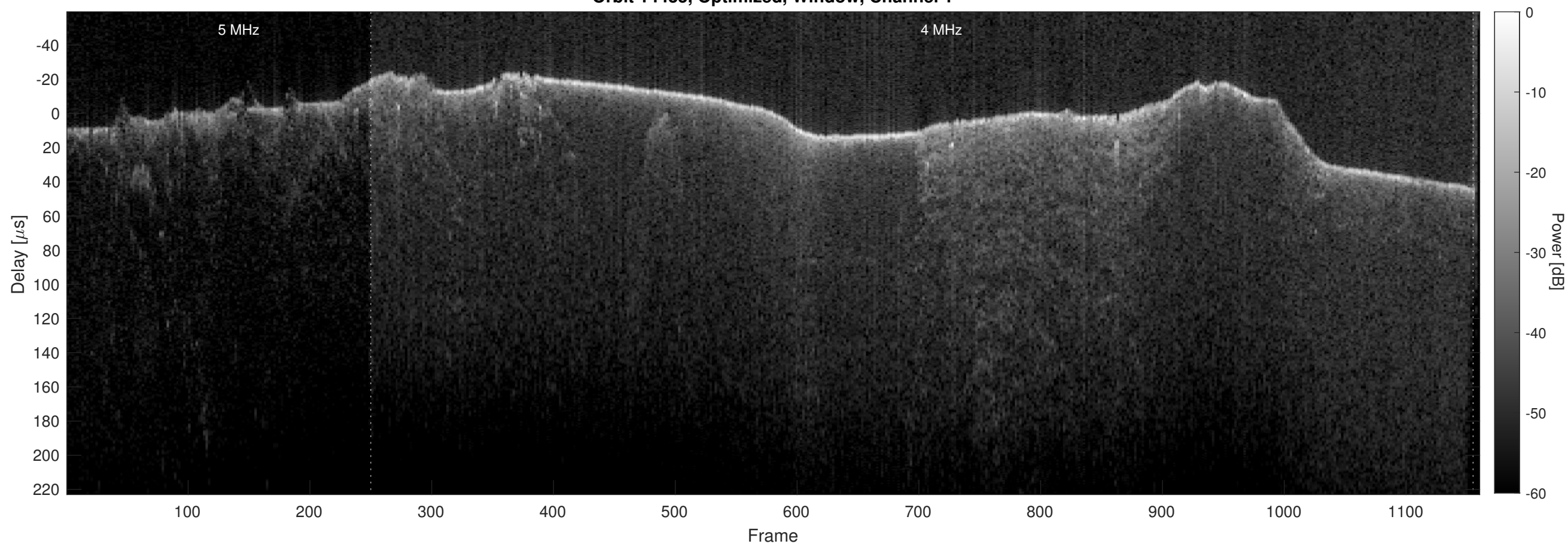
Orbit 14435, Optimized, Window, Channel 2
