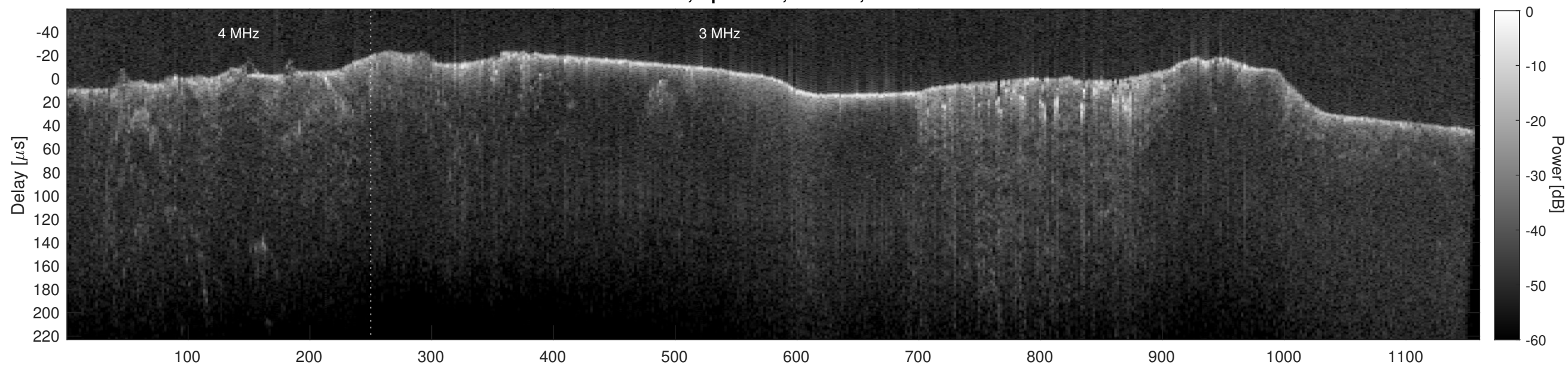
Orbit 14435, Cluttergram
