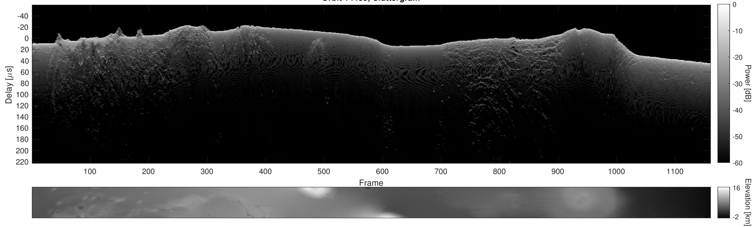
Orbit 14435, Cluttergram
