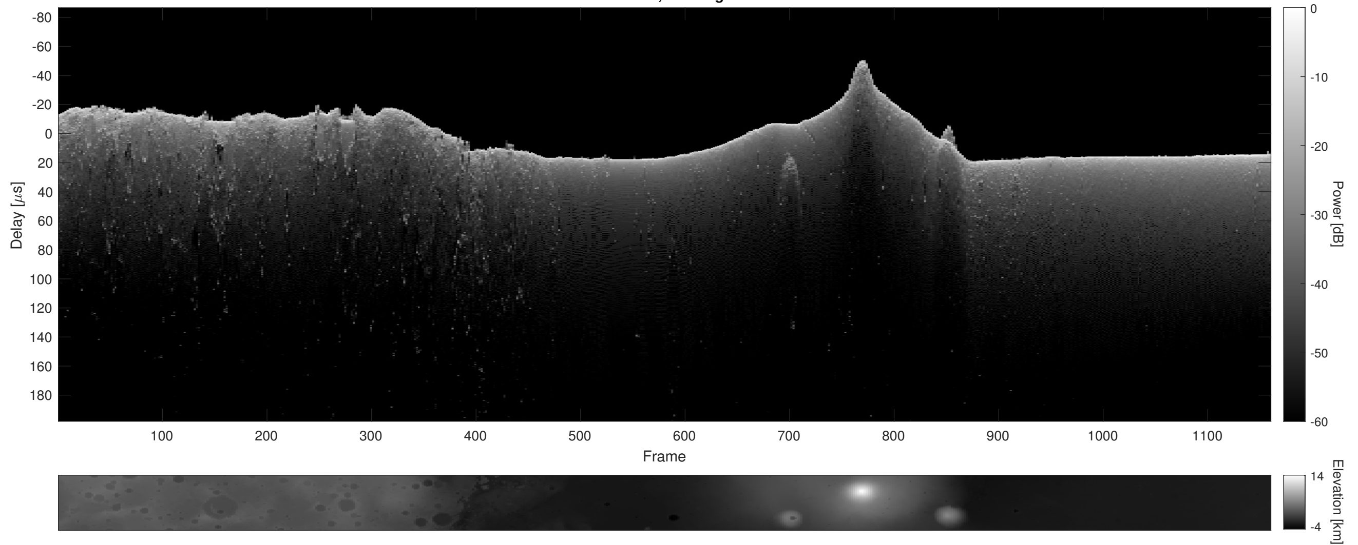
Orbit 14436, Cluttergram
