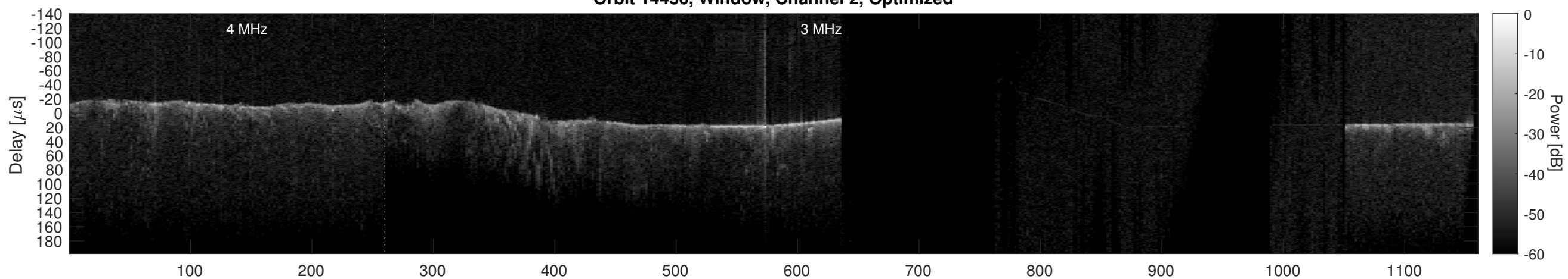
Orbit 14436, Cluttergram
