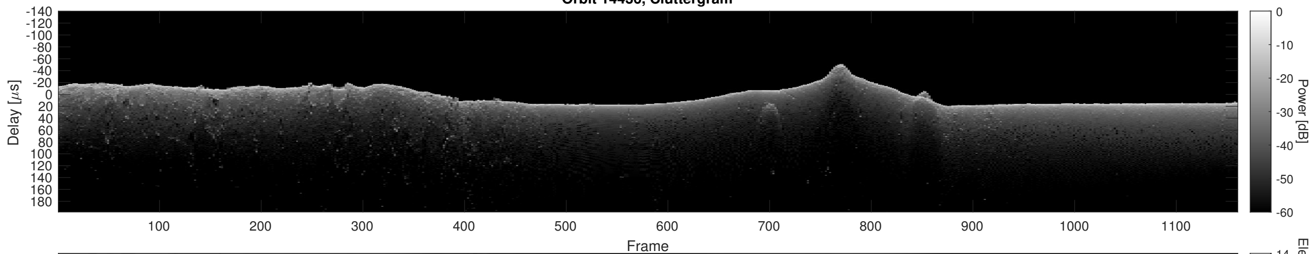
Orbit 14436, Cluttergram
