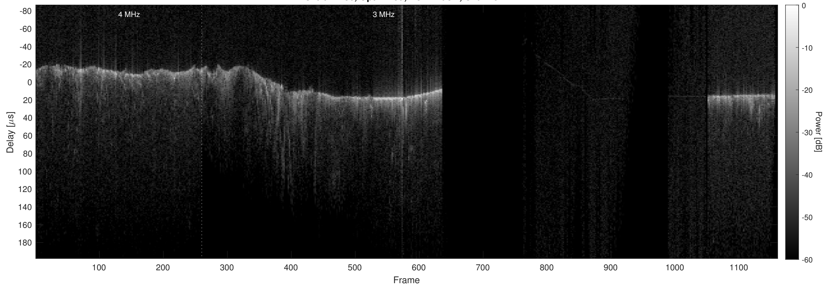
Orbit 14436, Optimized, No Window, Channel 2
