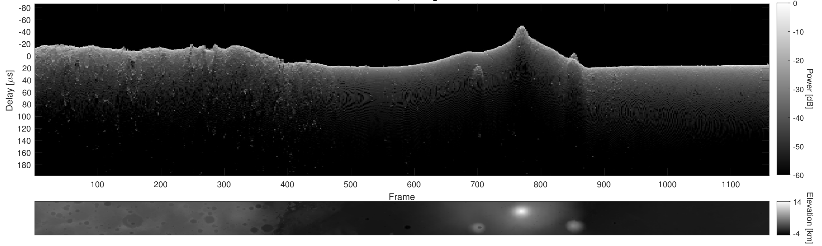
Orbit 14436, Cluttergram
