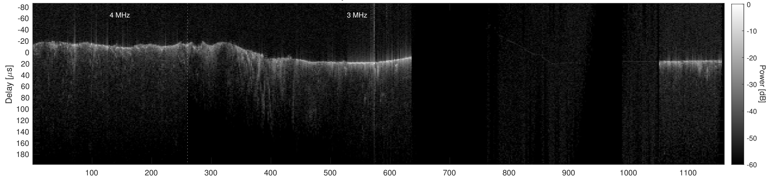
Orbit 14436, Cluttergram
