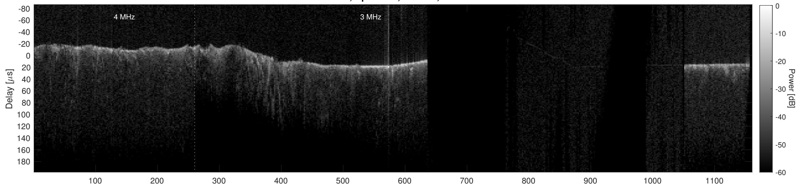
Orbit 14436, Cluttergram
