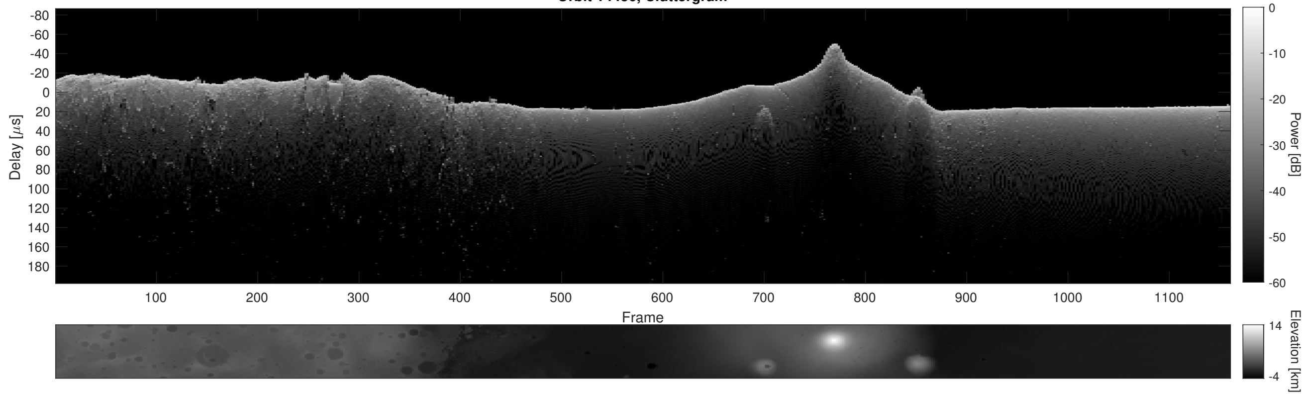
Orbit 14436, Cluttergram
