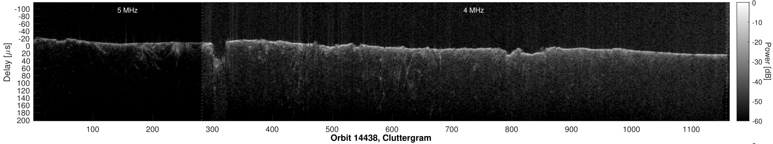
Orbit 14438, Window, Channel 1, Optimized
