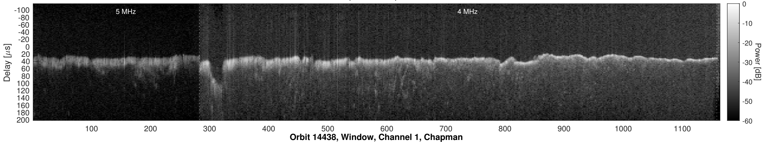
Orbit 14438, Channel 1, Uncorrected
