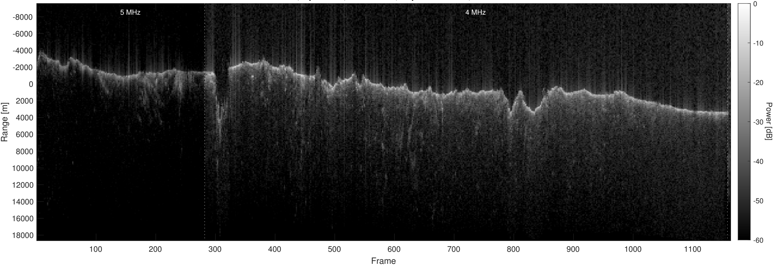
Orbit 14438, Optimized, No Window, Depth-Corrected, Channel 2
