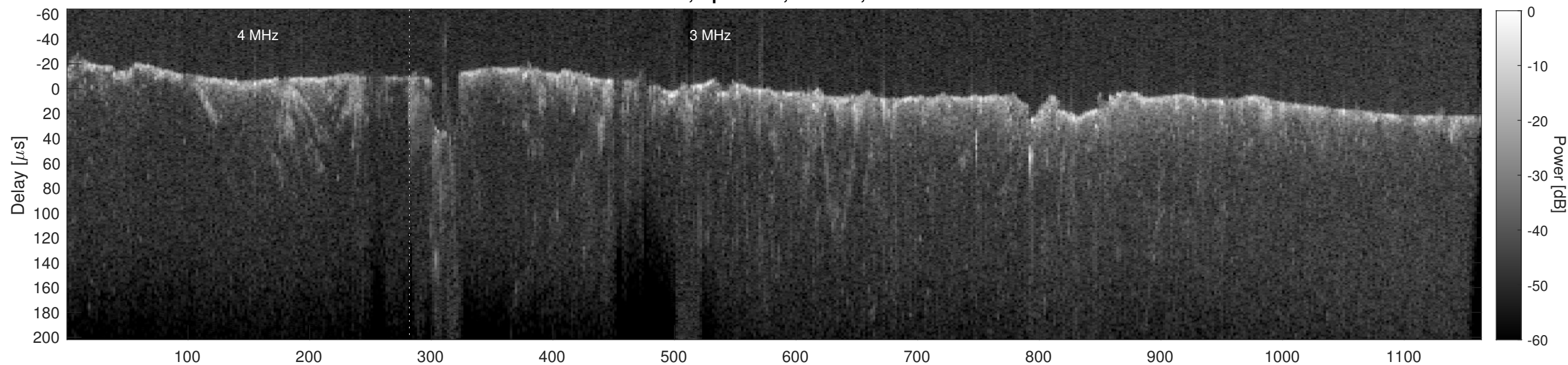
Orbit 14438, Cluttergram
