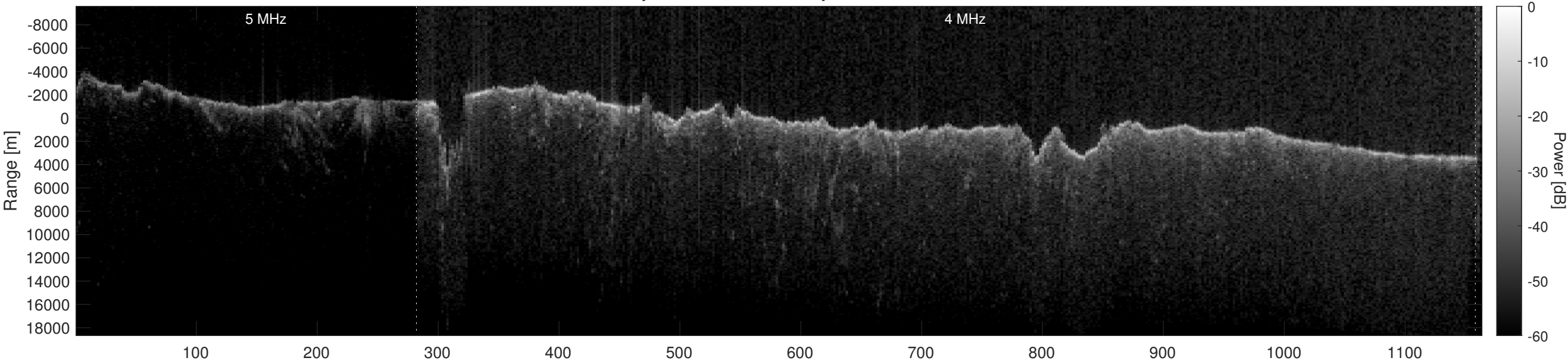
Orbit 14438, Optimized, Window, Depth-Corrected, Channel 2
