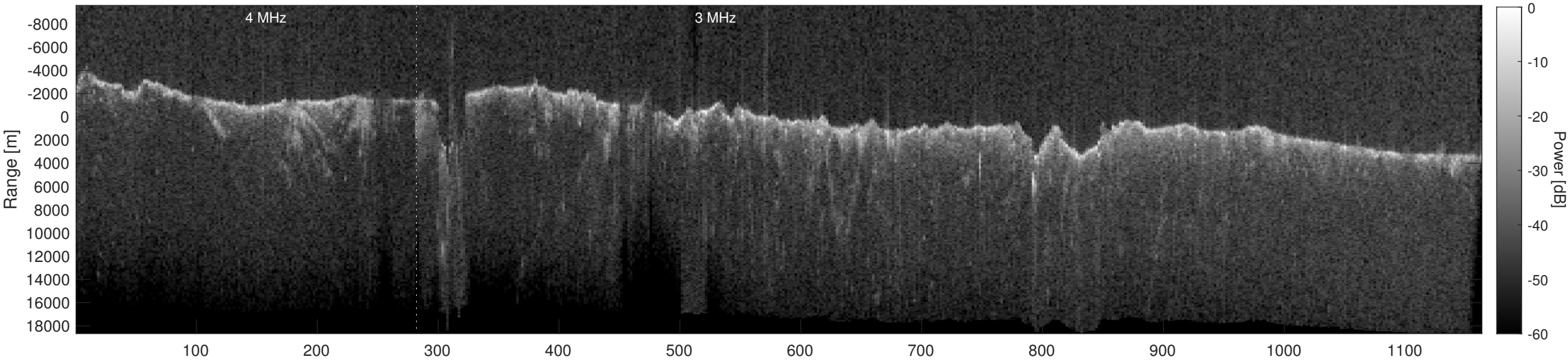
Orbit 14438, Depth-Corrected Cluttergram
