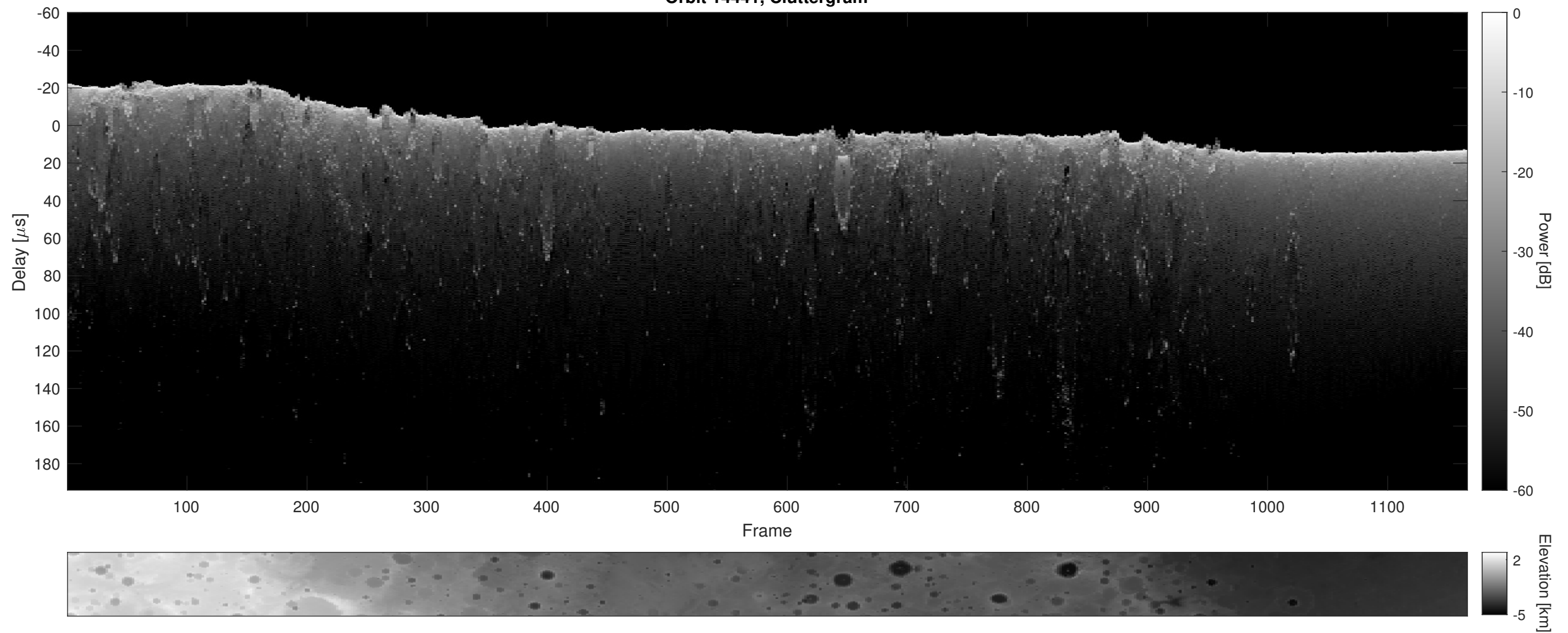
Orbit 14441, Cluttergram
