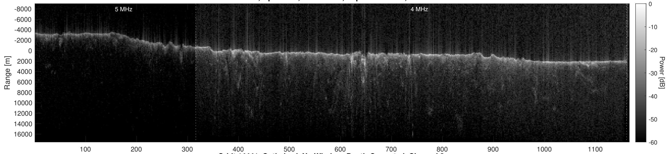
Orbit 14441, Optimized, No Window, Depth-Corrected, Channel 2
