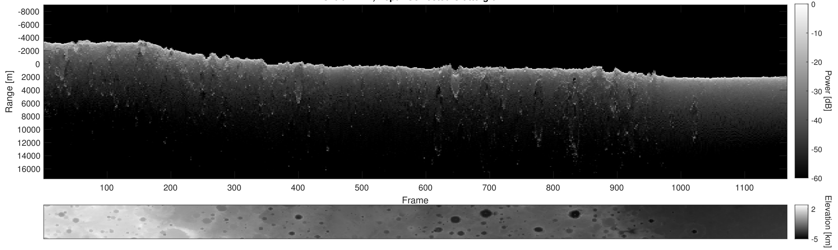
Orbit 14441, Depth-Corrected Cluttergram
