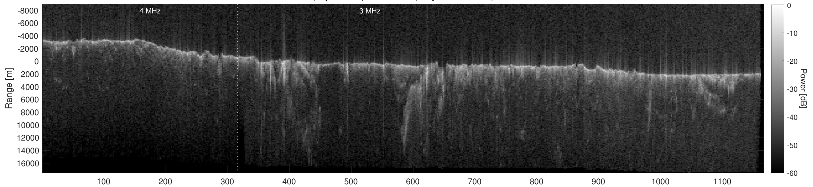
Orbit 14441, Depth-Corrected Cluttergram
