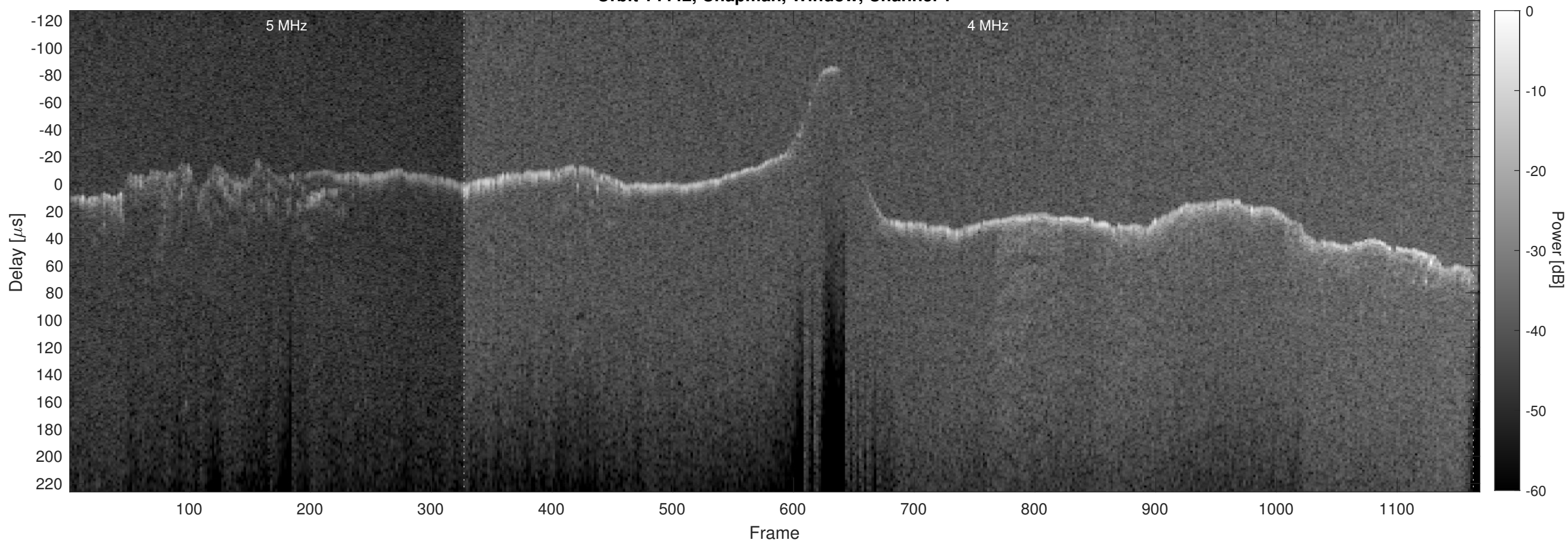
Orbit 14442, Chapman, Window, Channel 2
