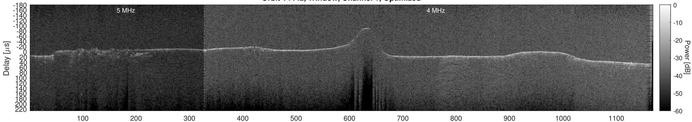
Orbit 14442, Cluttergram
