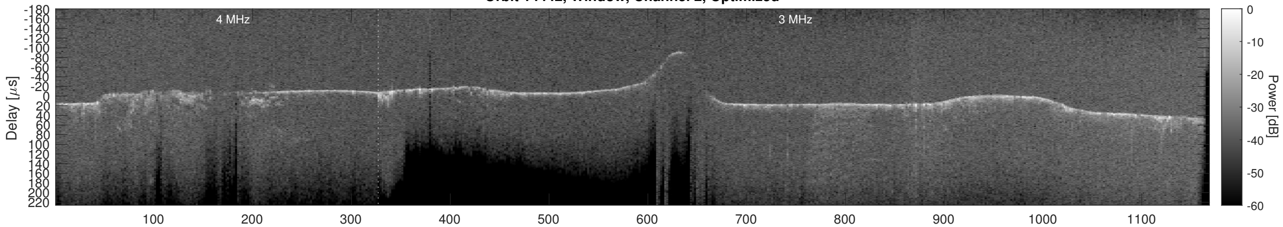
Orbit 14442, Cluttergram
