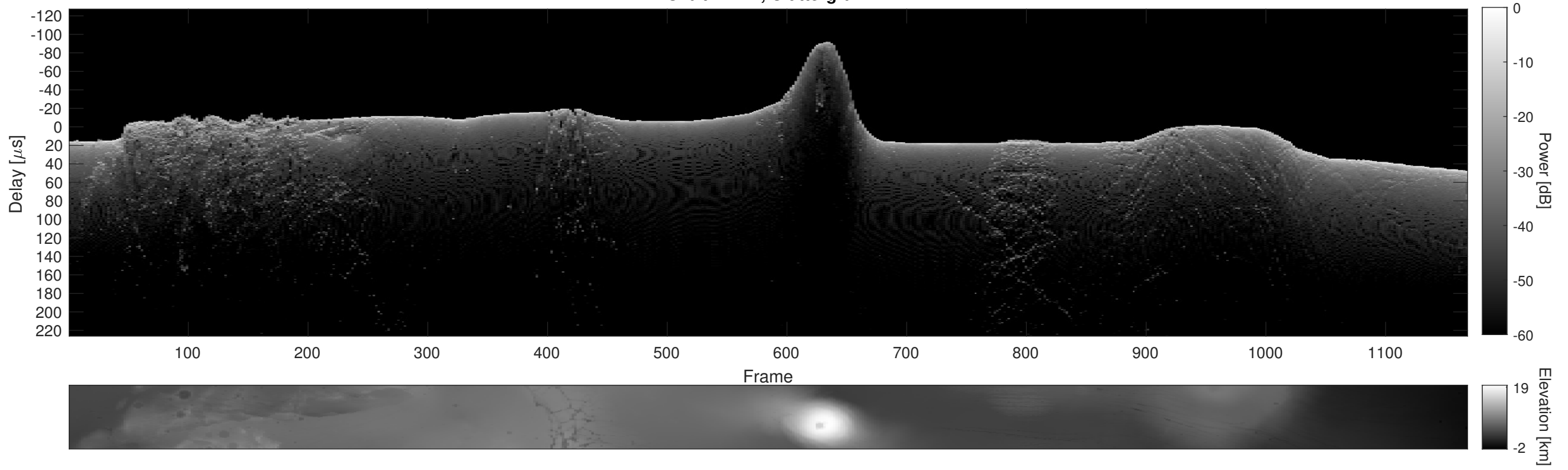
Orbit 14442, Cluttergram
