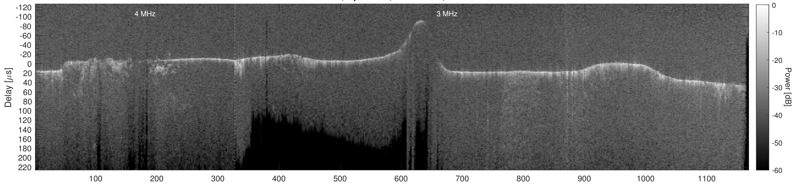
Orbit 14442, Cluttergram
