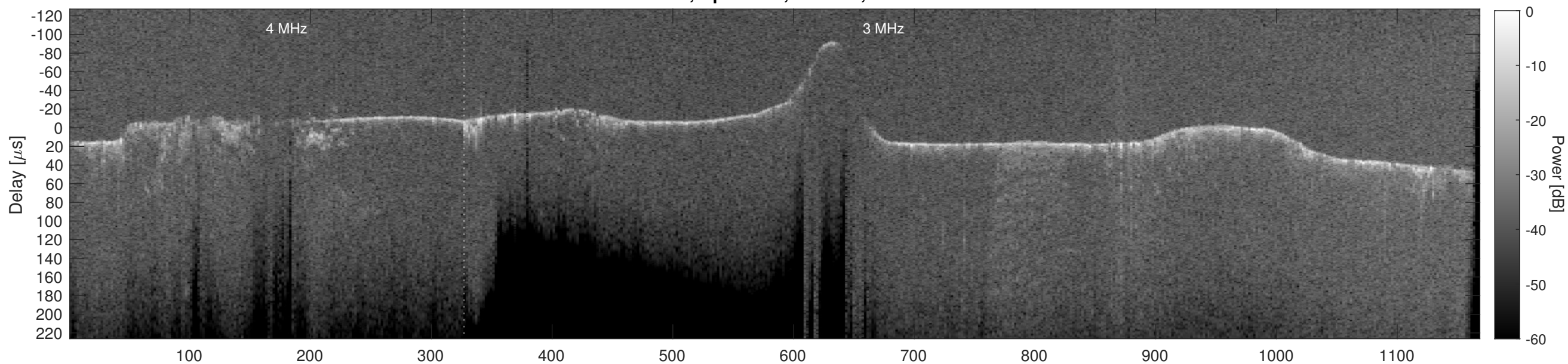
Orbit 14442, Cluttergram
