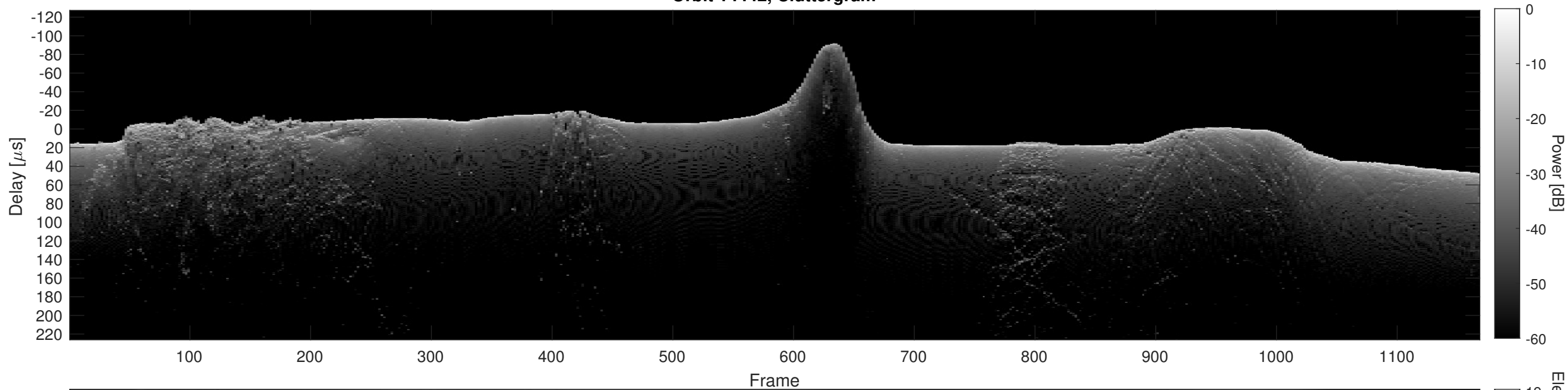
Orbit 14442, Cluttergram
