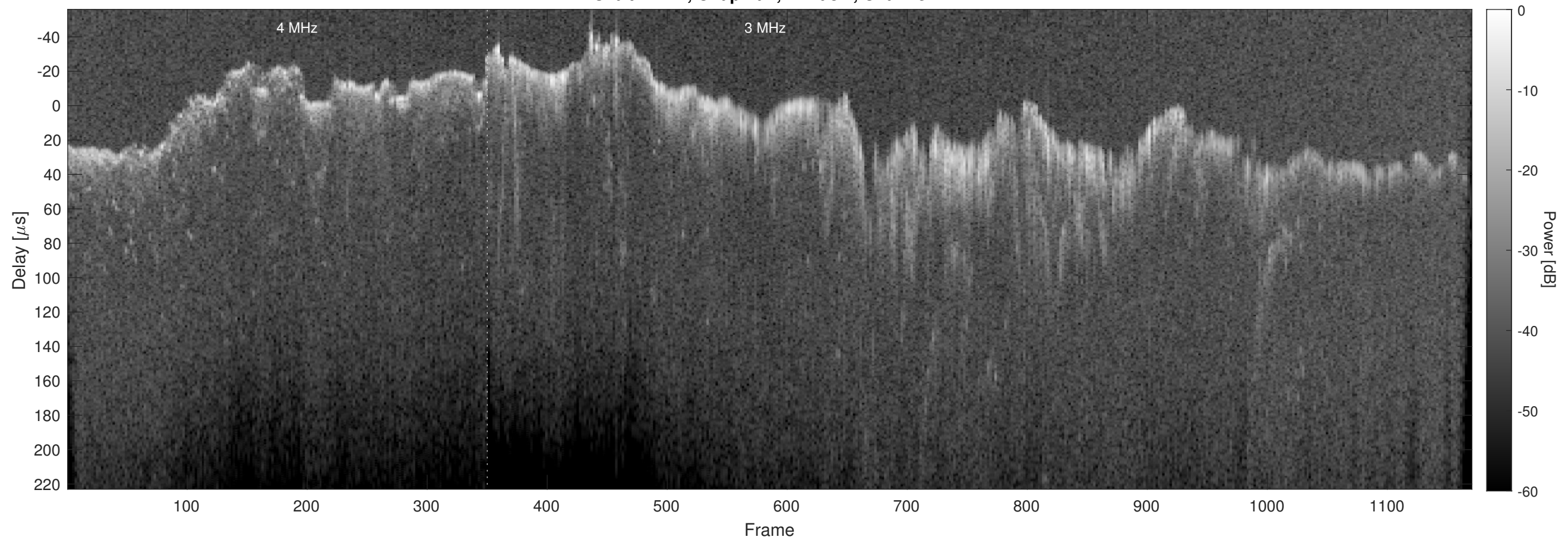
Orbit 14444, Chapman, Window, Channel 2
