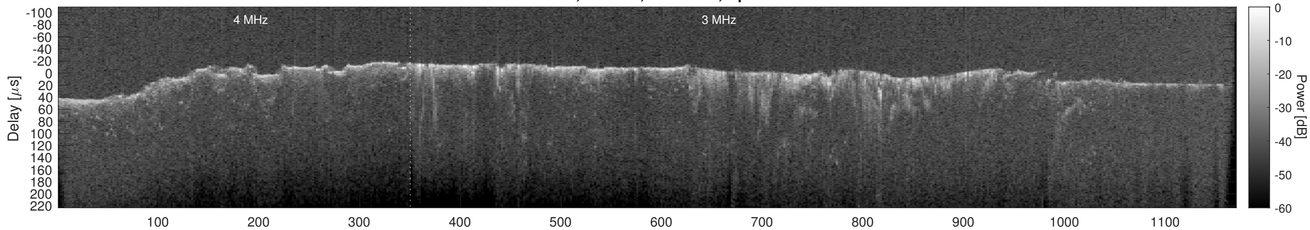
Orbit 14444, Cluttergram
