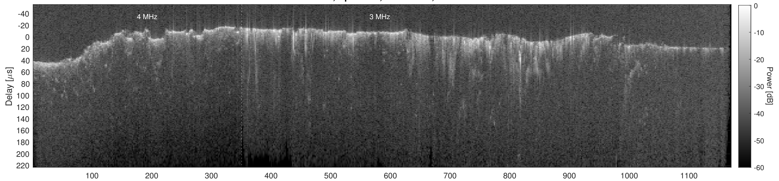
Orbit 14444, Cluttergram
