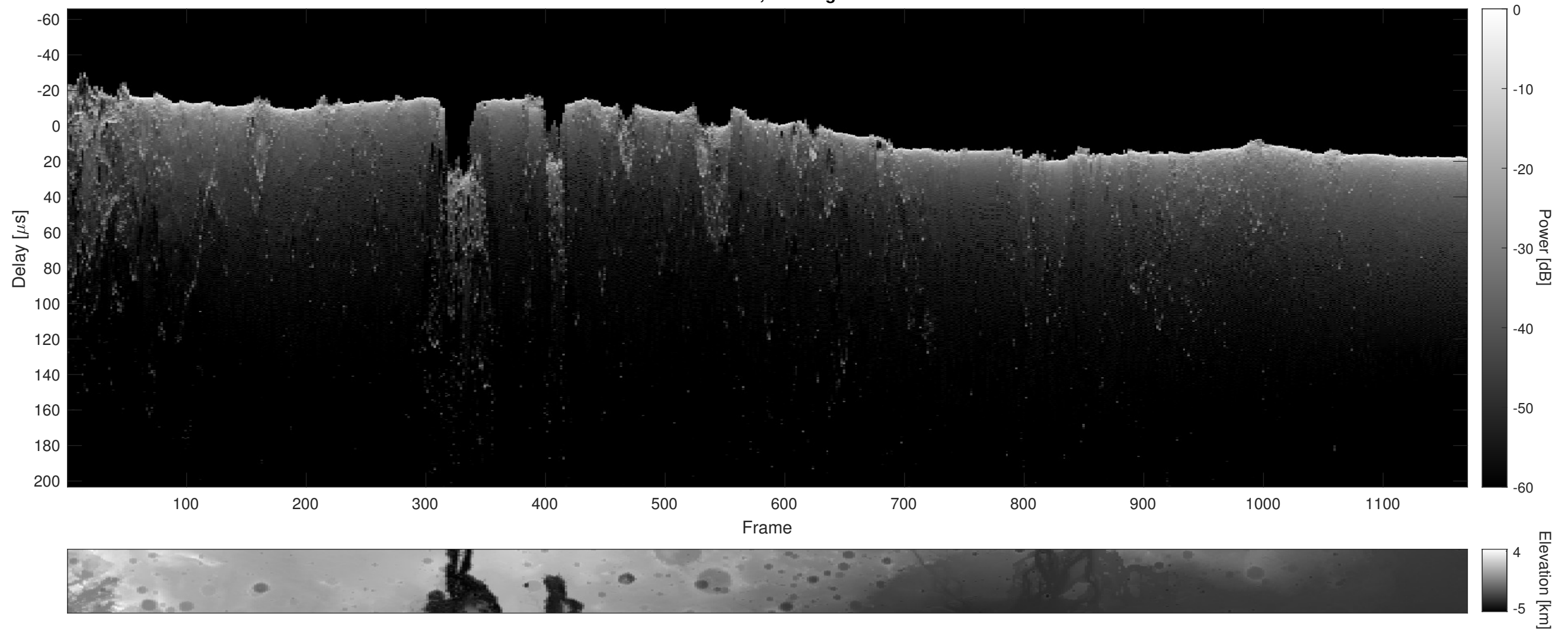
Orbit 14445, Cluttergram
