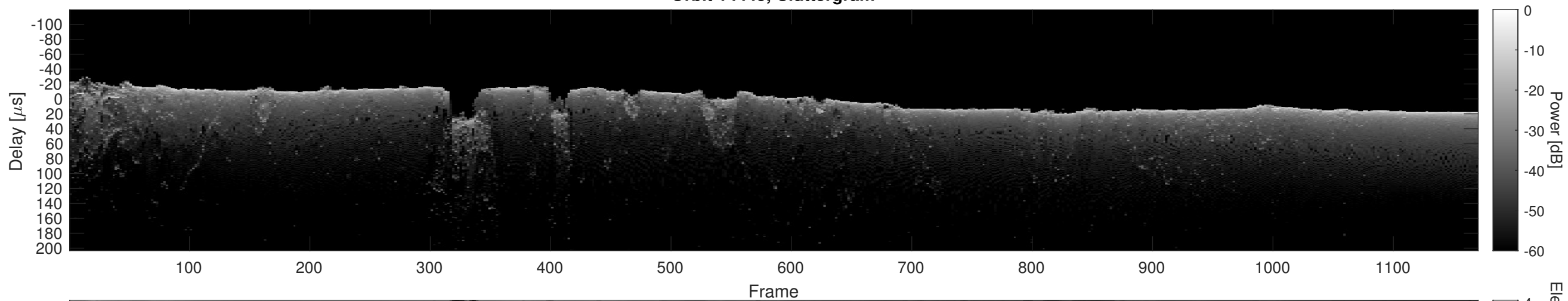
Orbit 14445, Cluttergram
