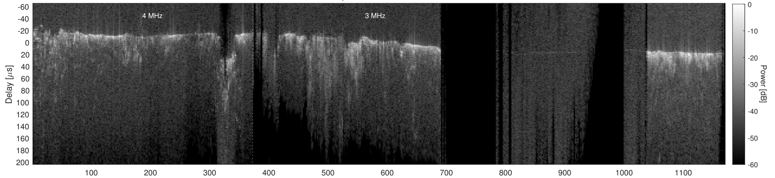
Orbit 14445, Cluttergram
