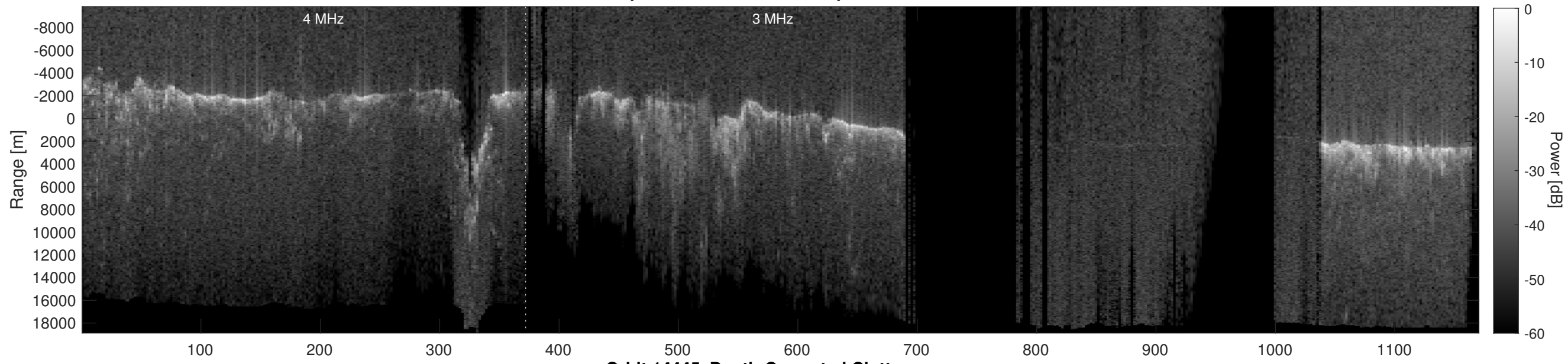
Orbit 14445, Depth-Corrected Cluttergram
