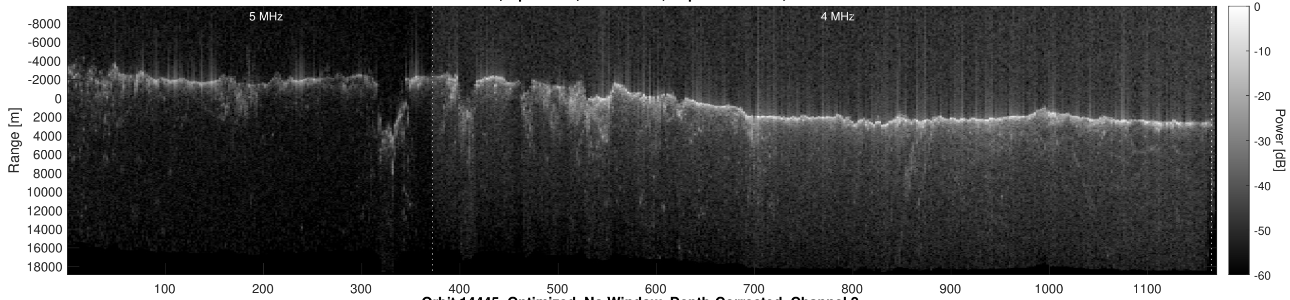
Orbit 14445, Optimized, No Window, Depth-Corrected, Channel 2
