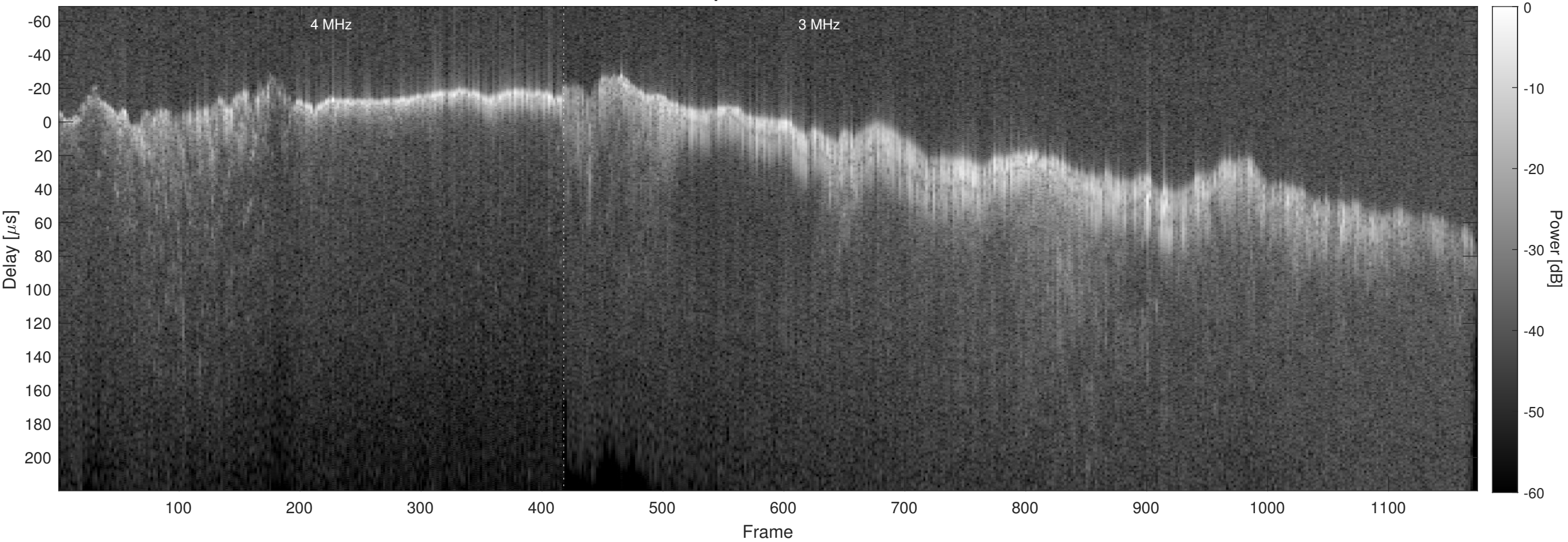
Orbit 14449, Chapman, No Window, Channel 2
