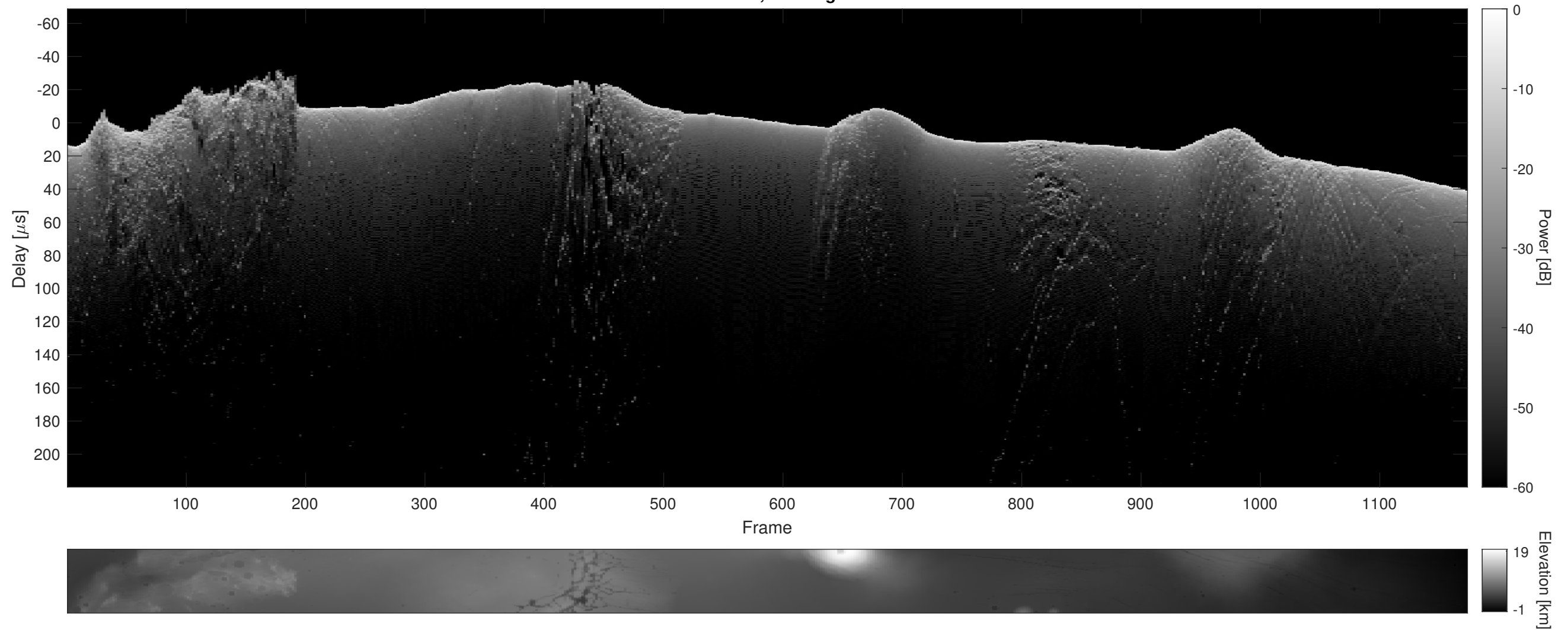
Orbit 14449, Cluttergram
