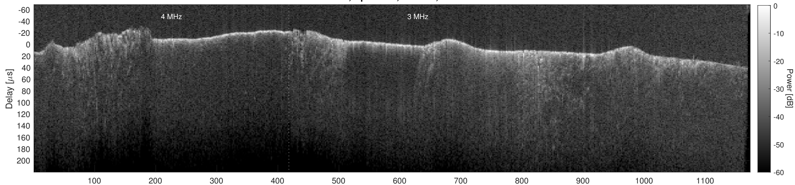
Orbit 14449, Cluttergram
