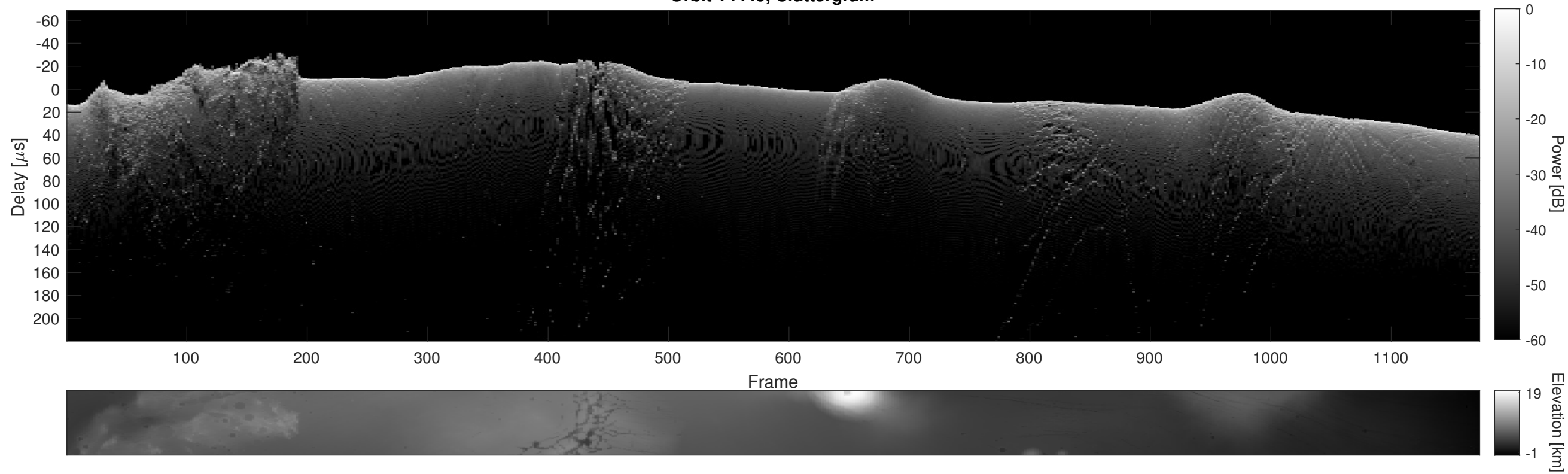
Orbit 14449, Cluttergram
