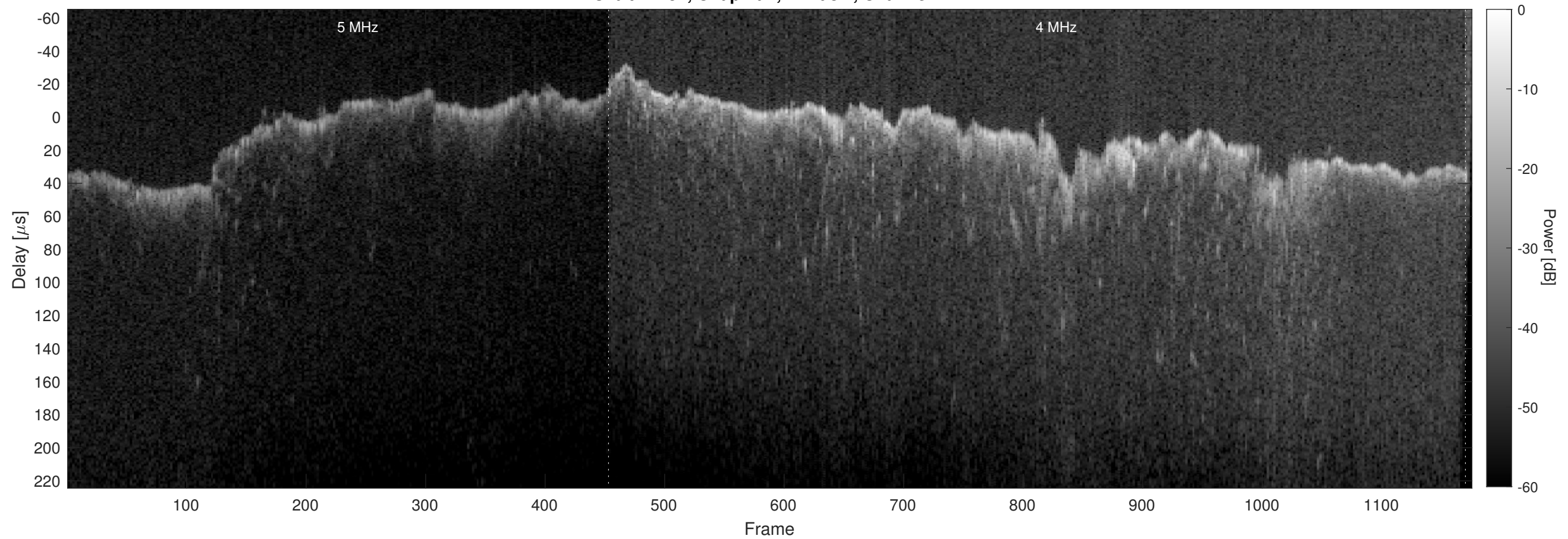
Orbit 14451, Chapman, Window, Channel 2
