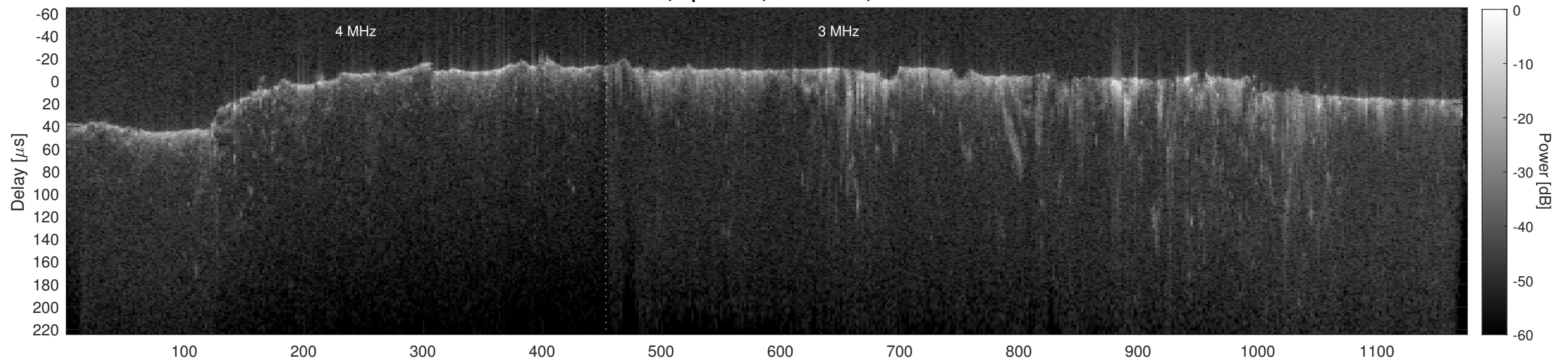
Orbit 14451, Cluttergram
