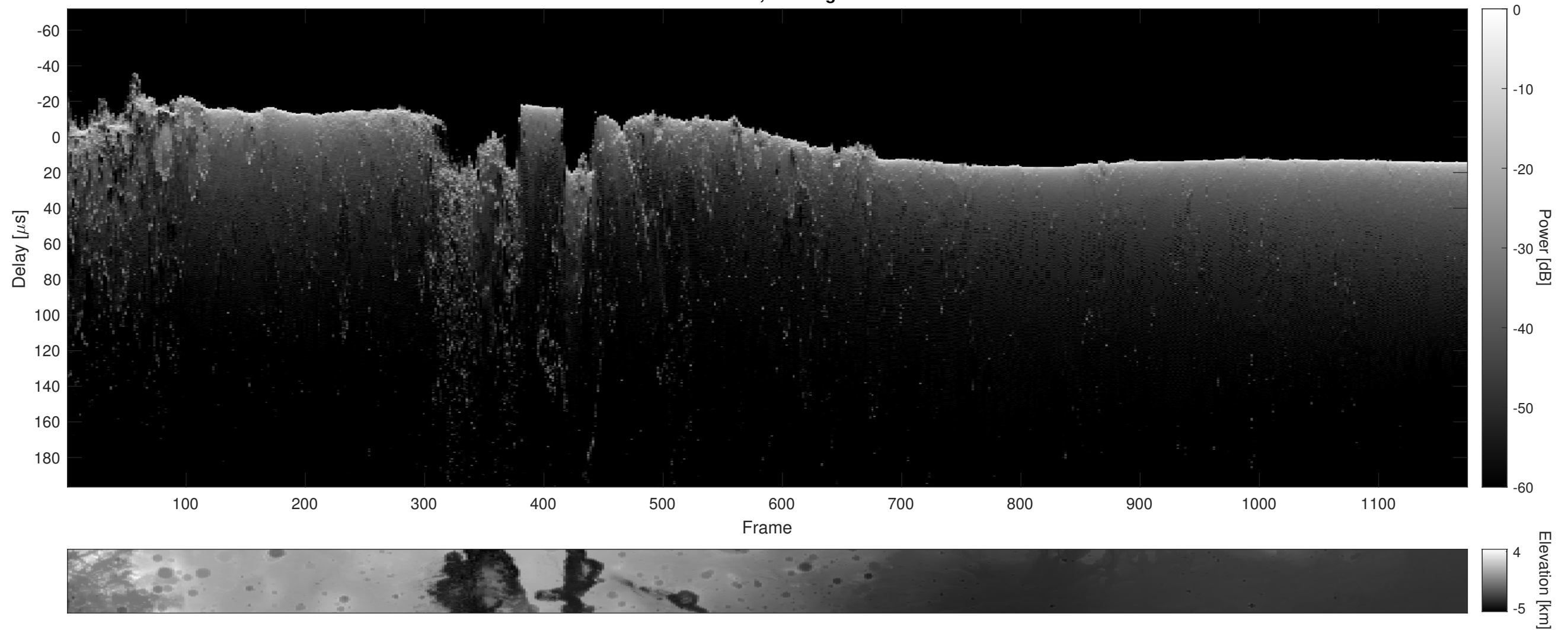
Orbit 14452, Cluttergram
