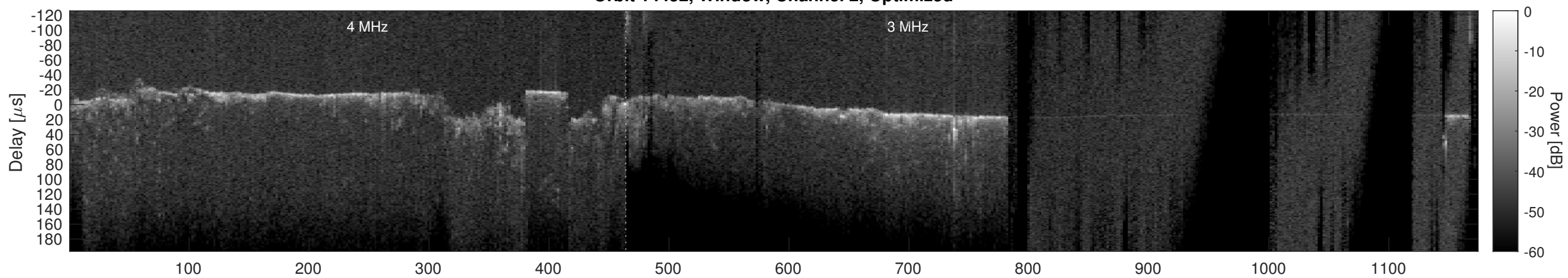
Orbit 14452, Cluttergram
