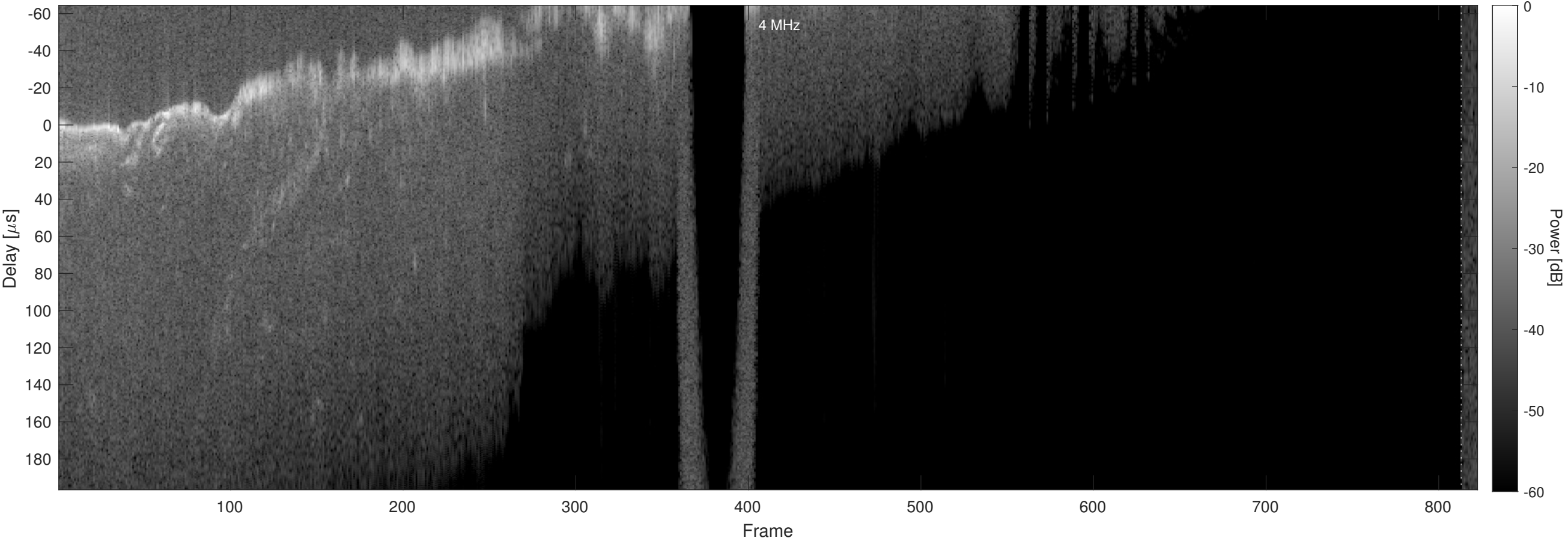
Orbit 14678, Chapman, No Window, Channel 2
