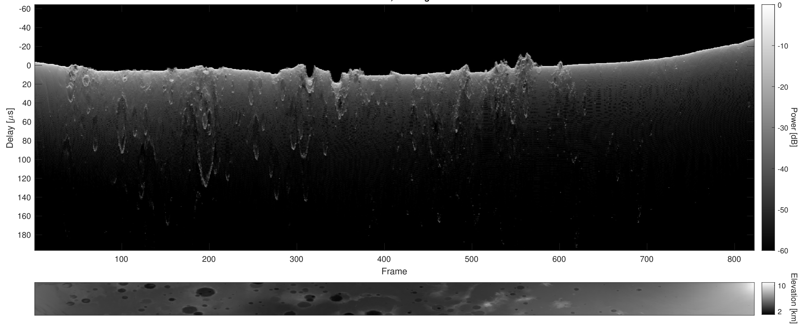
Orbit 14678, Cluttergram
