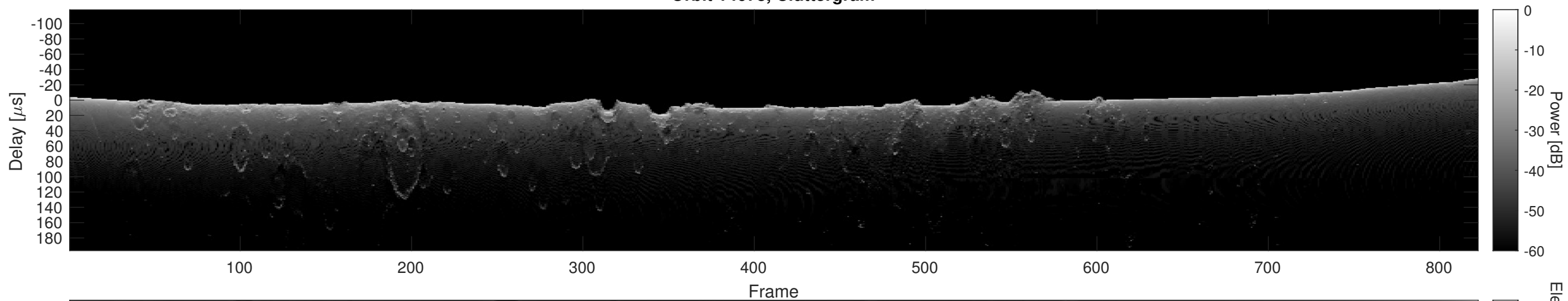
Orbit 14678, Cluttergram
