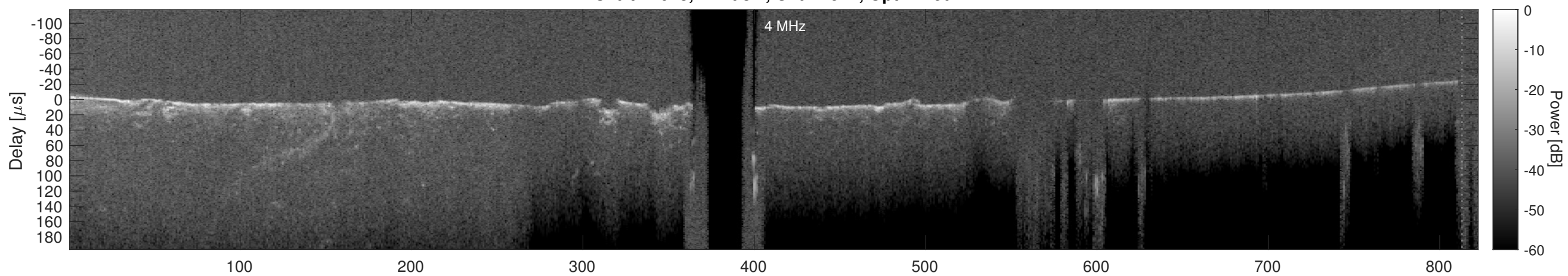
Orbit 14678, Cluttergram
