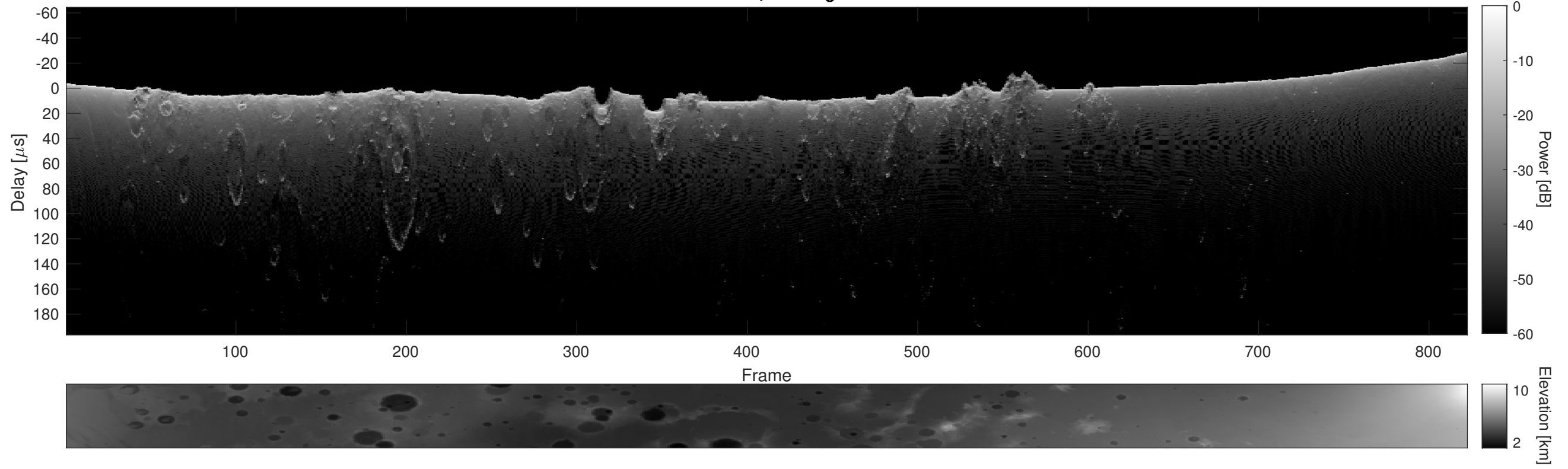
Orbit 14678, Cluttergram
