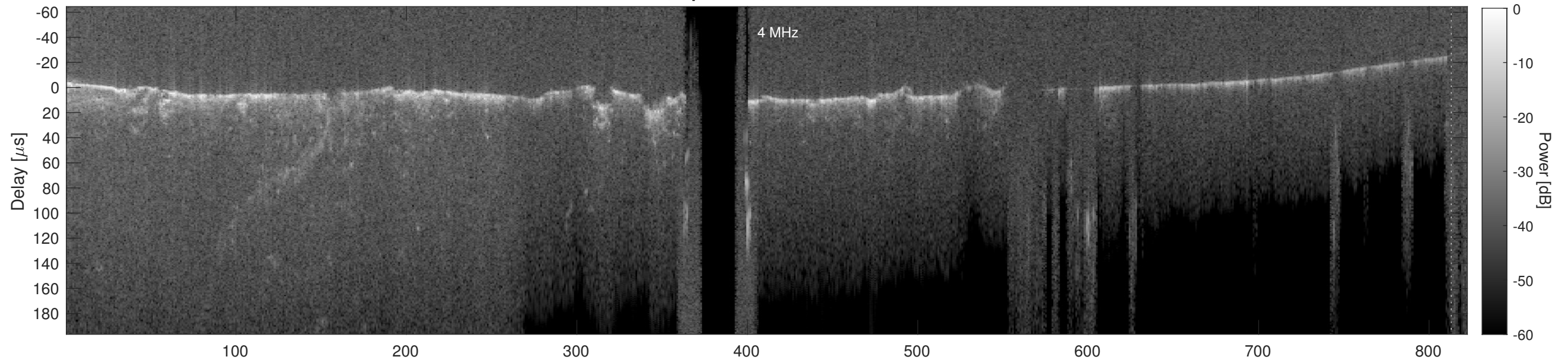
Orbit 14678, Cluttergram
